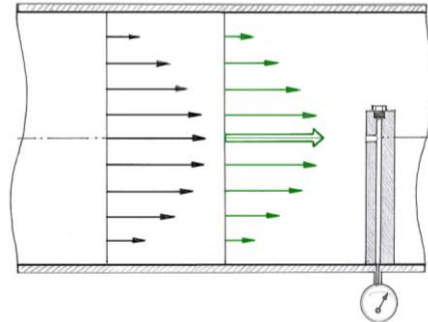
pressure optimized
